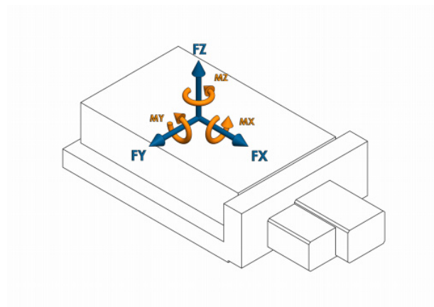
LOAD DIRECTIONS
